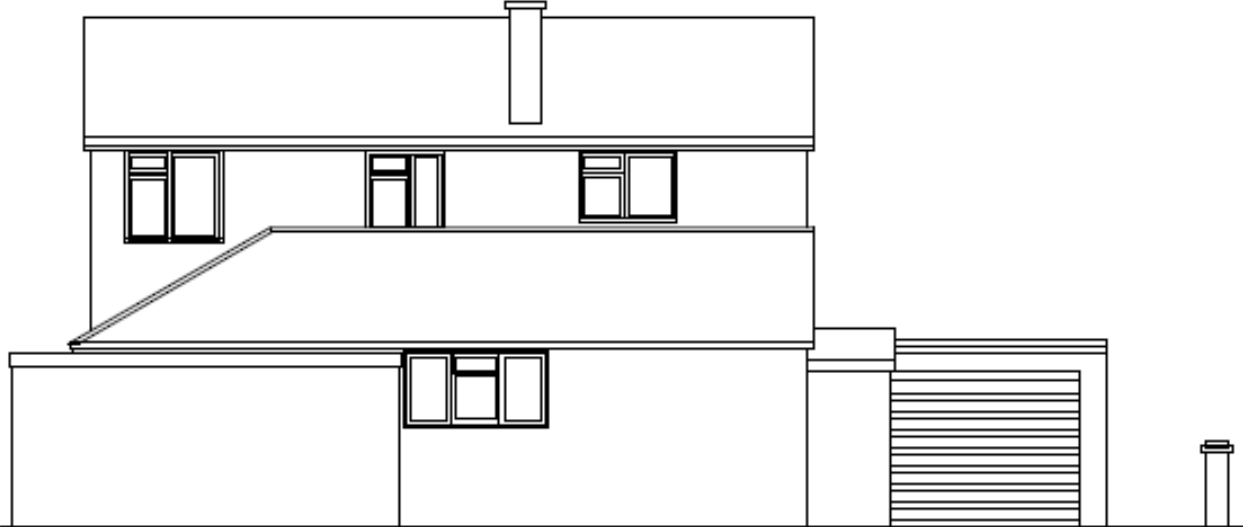
North elevation
